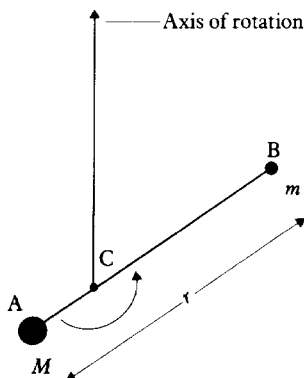
1.17 Bohr model with finite nuclear mass.
